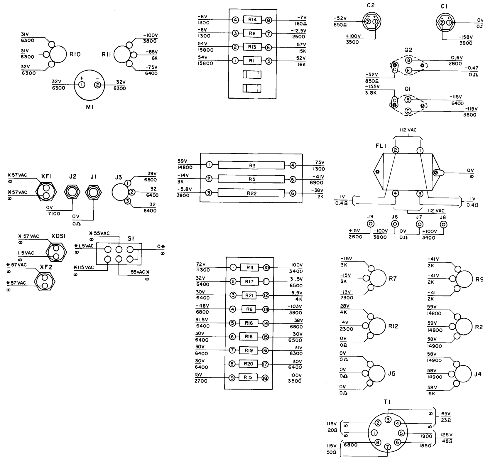
Figure 7-3. Chassis assembly 3A1, voltage and resistance diagram.
