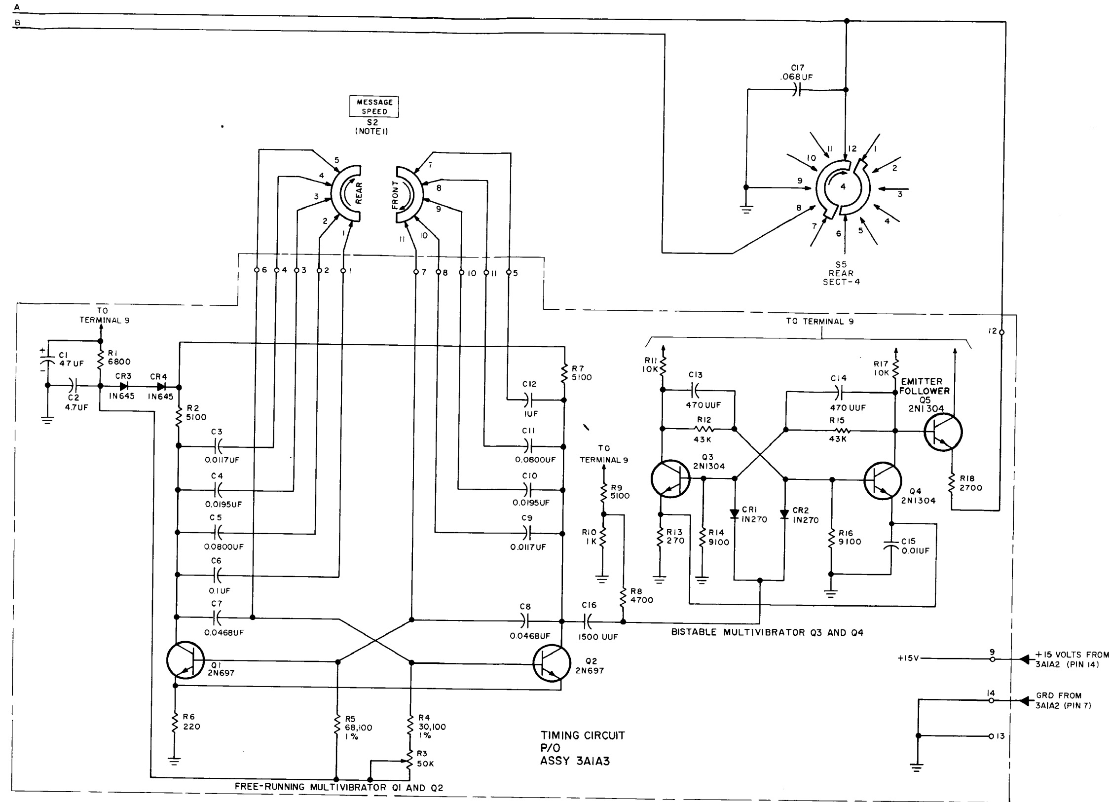
Figure 7-4 (2) Test Set, Relay TS-336/UGM-1, schematic diagram.
