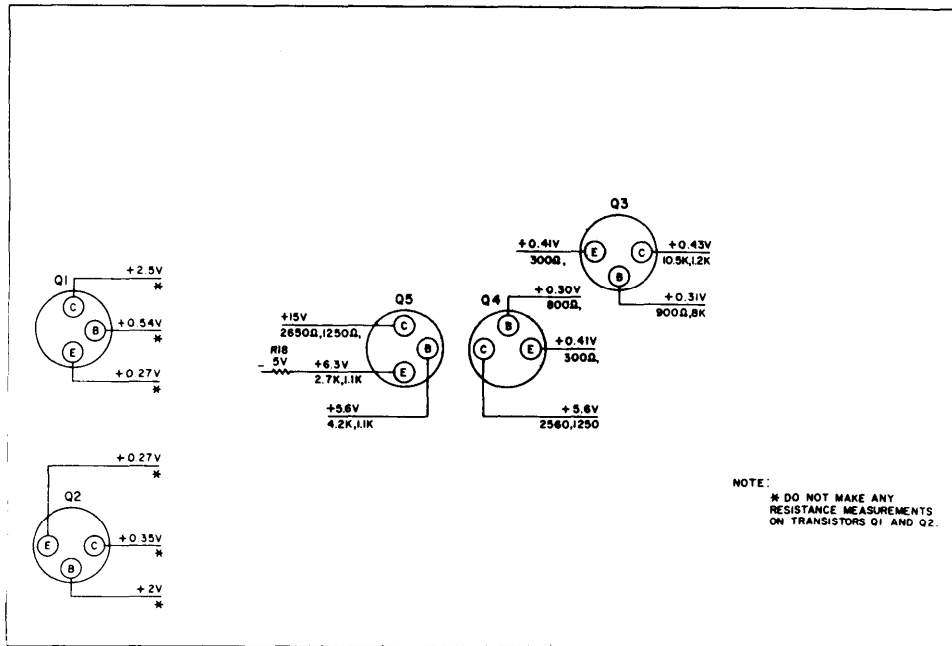
Figure 3-8. Timing circuit assembly 3A1A3, voltage and resistance diagram.
