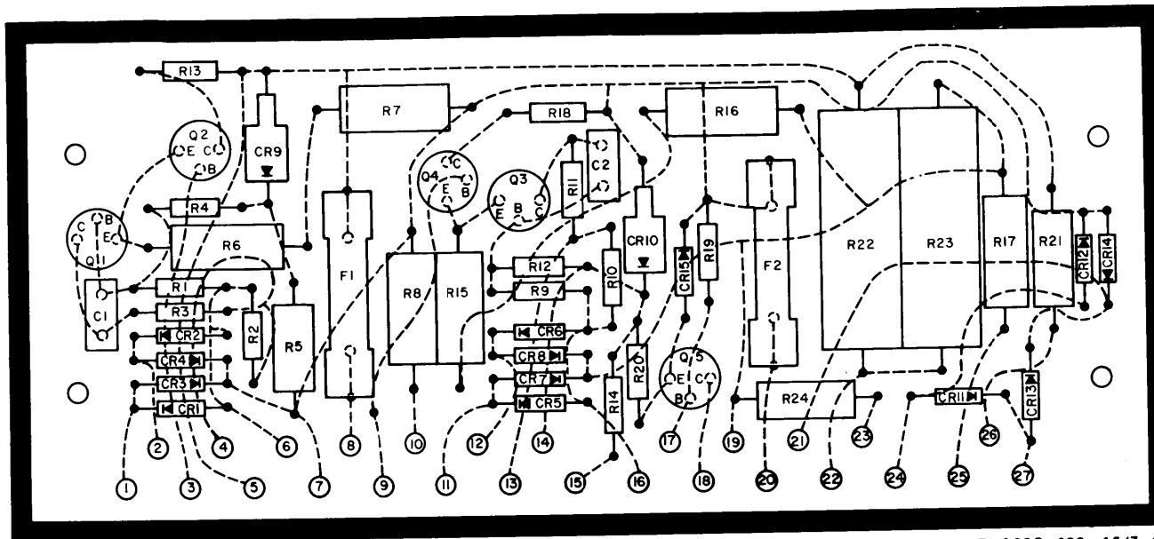
Figure 3-1. Power supply assembly SA1A2, parts locations.
